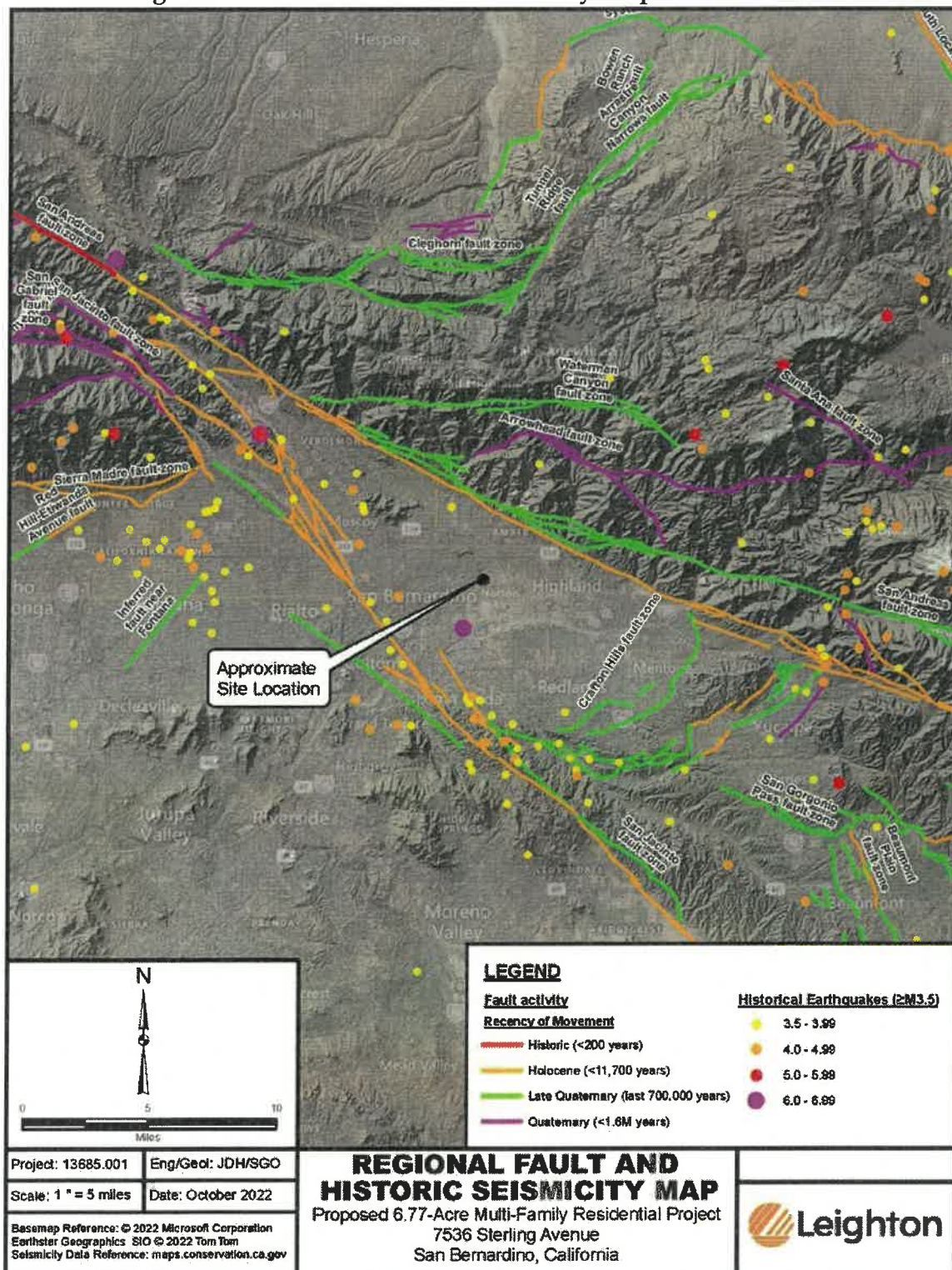
Exhibit 4.7-1 Regional Fault and Historical Seismicity Map
