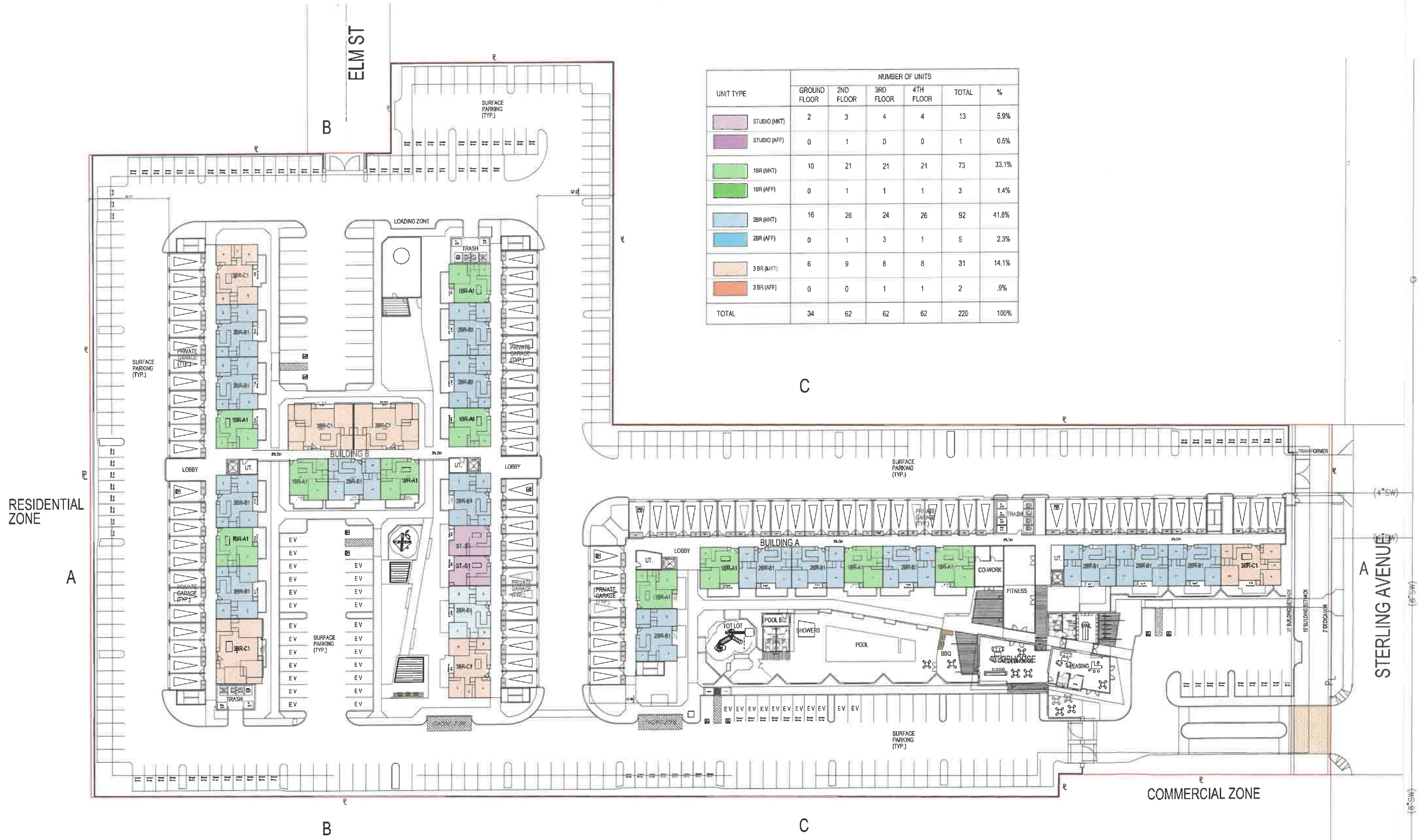
SITE PLAN/GROUND FLOOR BUILDING PLAN - UNIT MIX ARCHITECTURAL ENTITLEMENT SET
